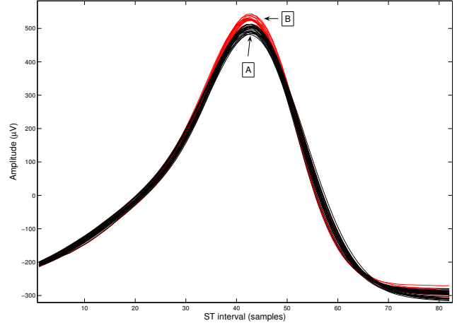
Figure 1. Time-aligned extracted ST-T segments for a single time series of 30 seconds. Note the two different beats types, separated by an average amplitude of 30 \mu V .
